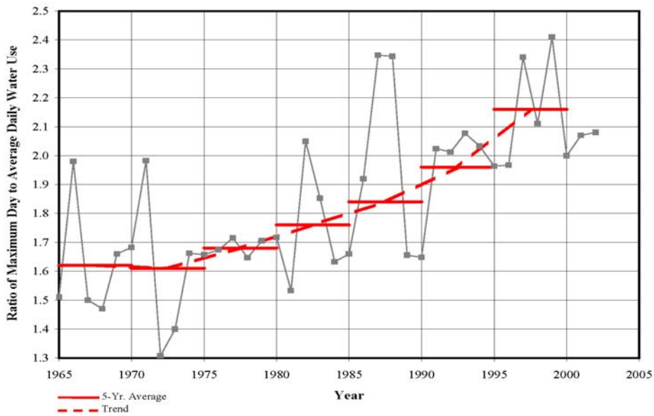
Figure 4. Maximum-Day-to-Average-Daily Water Use Ratio
